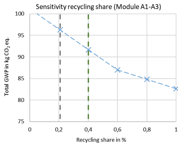
Fig. 6-1: Total GWP of the window manufacturing module (A1–A3) depending on the recycle content
